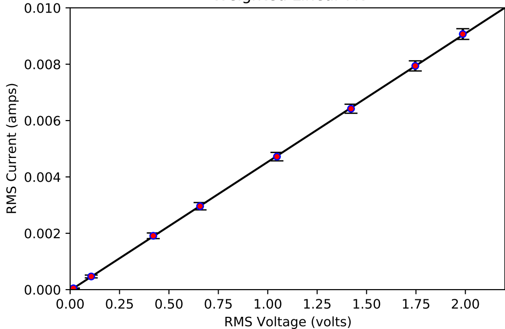
Weighted Linear Fit
